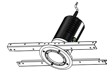
Shield as-bracket (2440010795)
